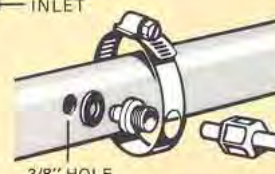
Saddle Clamp Assembly. For easy installation in system piping.
